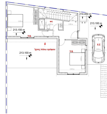
1 1st floor 1 : 100
