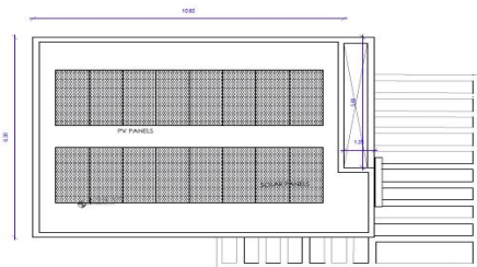
ROOF PLAN SC:1:100
