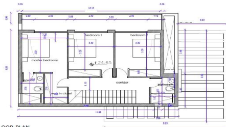
FIRST FLOOR PLAN SC:1:100
