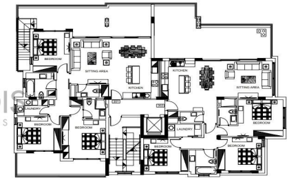
Third Floor
