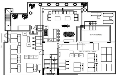
Roof Plan
