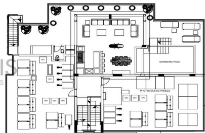
Roof Plan
