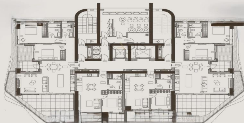
4th-6th floors layout plan
