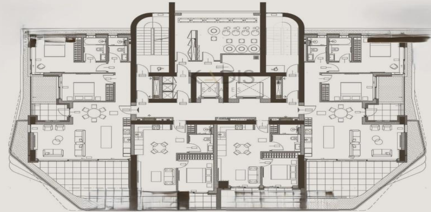
4th-6th floors layout plan
