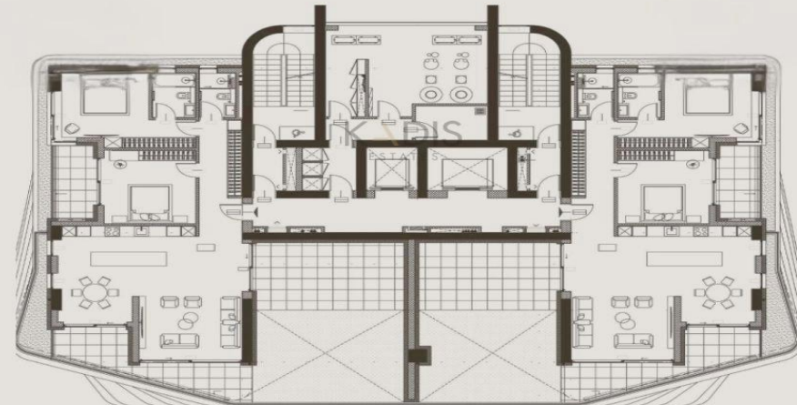
1 2nd floor layout plan
