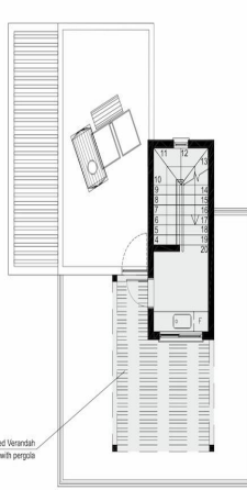
ROOF FLOOR
