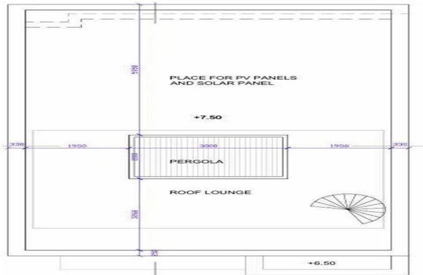
ROOF PLAN
