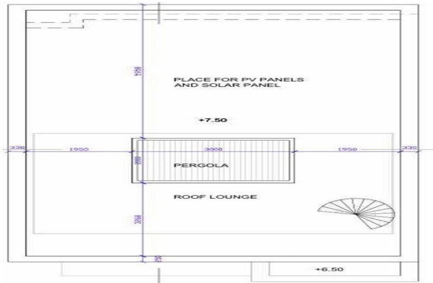
ROOF PLAN
