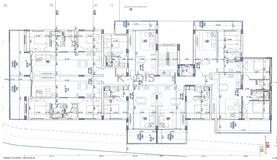
FIRST FLOOR - BLOCK B 1:100
