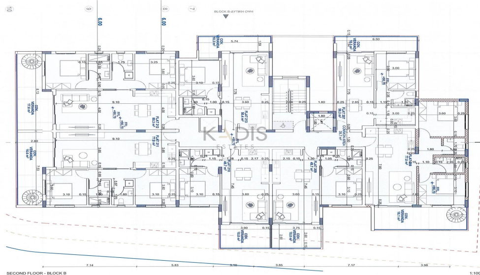
SECOND FLOOR - BLOCK B 1:100
