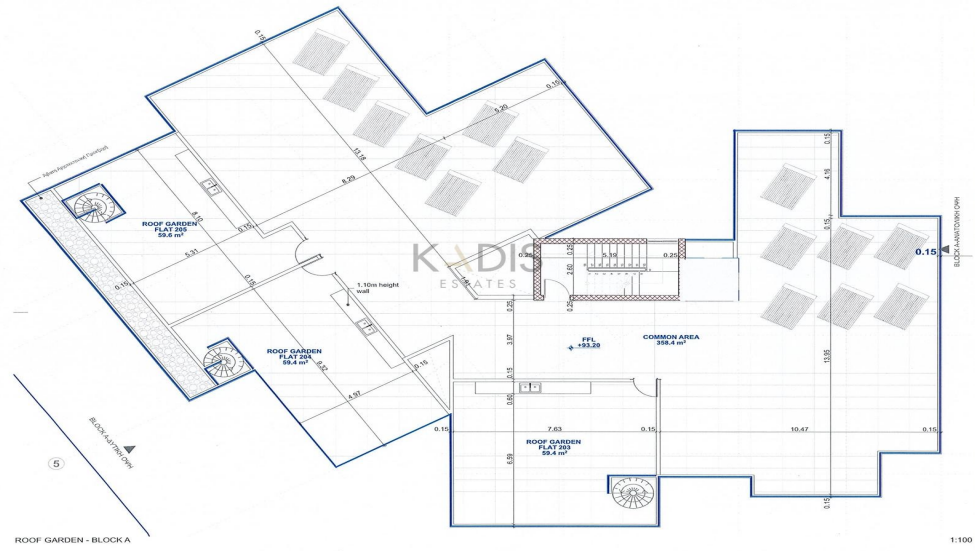
ROOF GARDEN - BLOCK A 1:100
