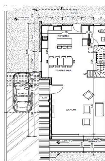
VILLAS NO. 1, 3, 5 & 6 (TYPE A1/A2)
