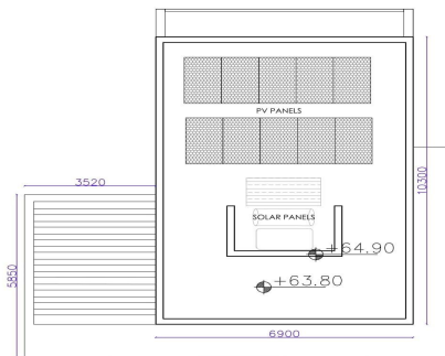
ROOF PLAN SCALE 1:100
