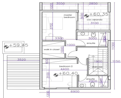
FIRST FLOOR SCALE 1:100
