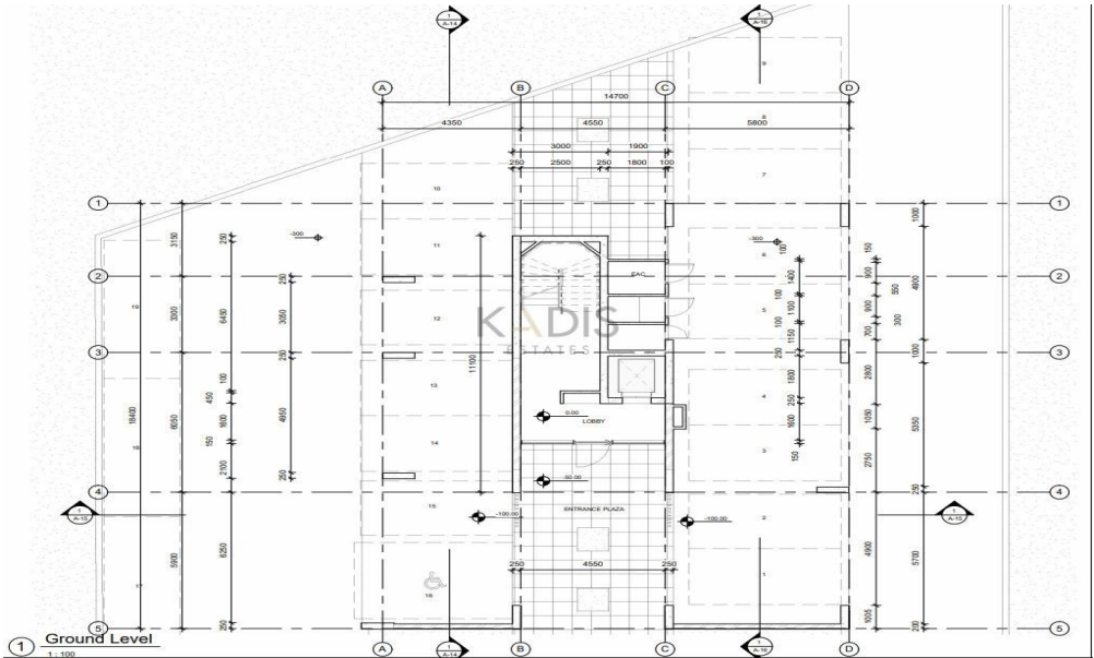
① Ground Level 1:100
