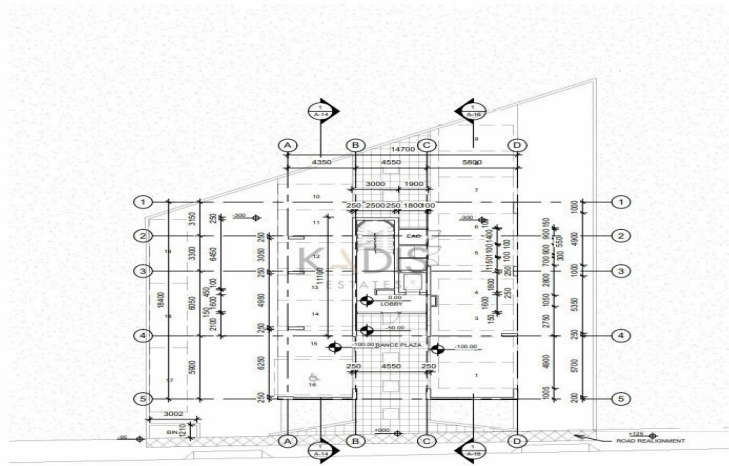
① Ground Level (Full Plot) 1:200
