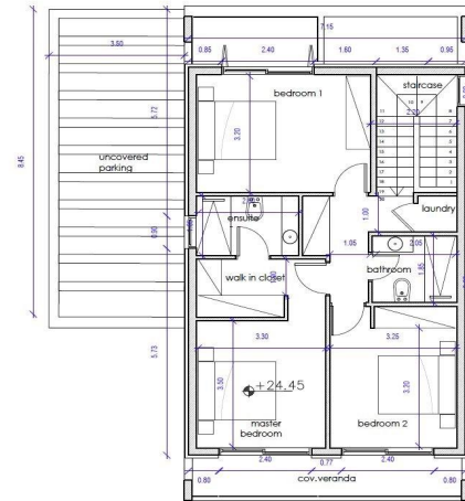
FIRST FLOOR PLAN SC:1:100
