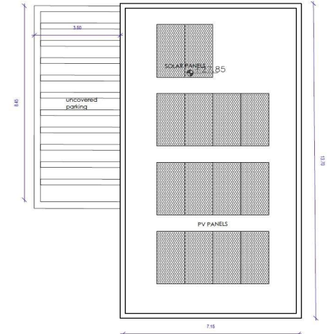
ROOF PLAN SC:1:100
