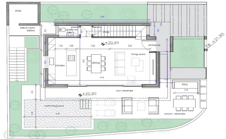
GROUND FLOOR PLAN SC:1:100
