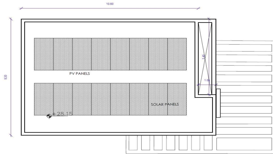
ROOF PLAN SC:1:100
