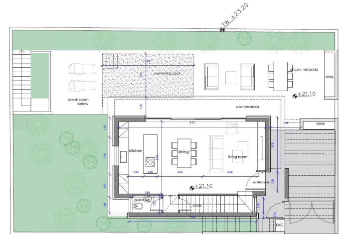
GROUND FLOOR PLAN SC:1:100
