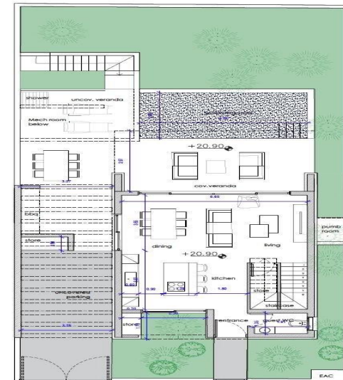
GROUND FLOOR PLAN SC:1:100
