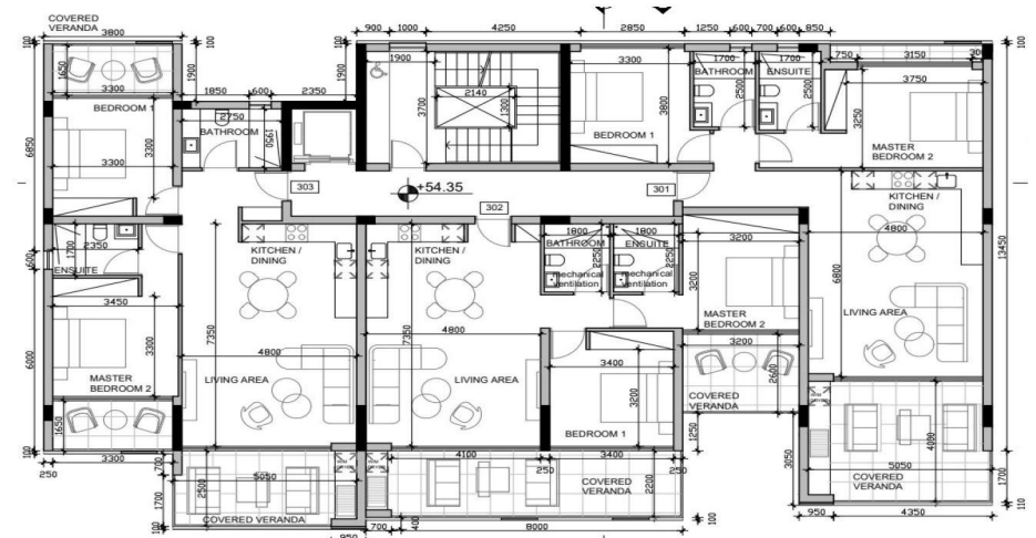
Block D - Third Floor
