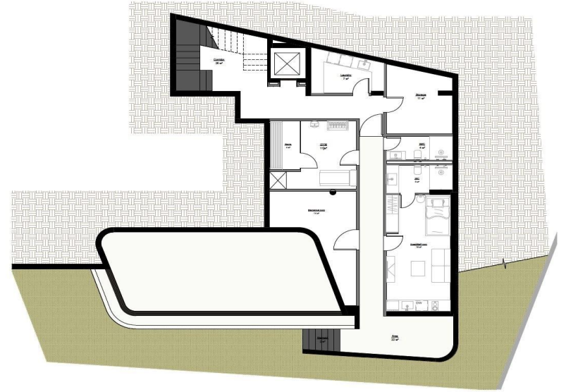
BASEMENT
