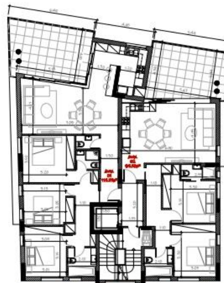
FLOOR PLANS [1st-4th Floor] - 2+3 BEDROOMS FLATS
