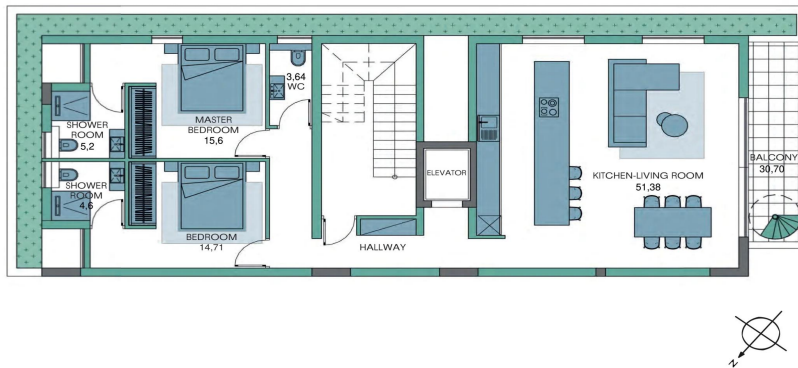
FLOOR PLAN 3
