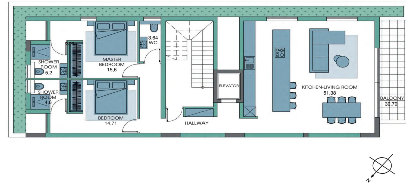
FLOOR PLAN 2
