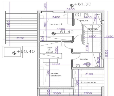
FIRST FLOOR SCALE 1:100
