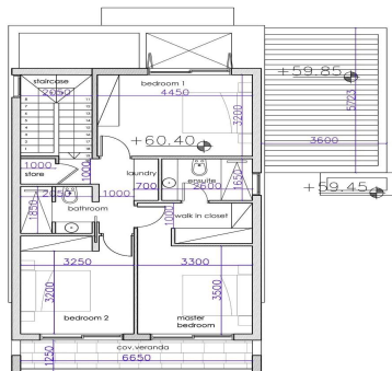
FIRST FLOOR SCALE 1:100
