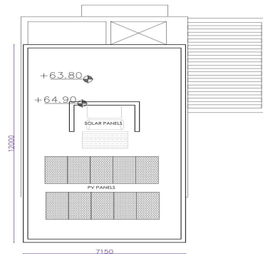
ROOF PLAN SCALE 1:100
