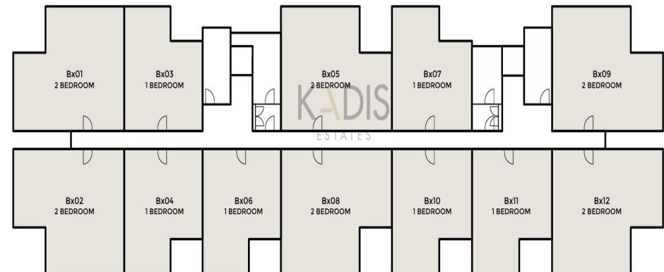
BLOCK B Typical Layout FLOORS: 1 ST - 5 TH
